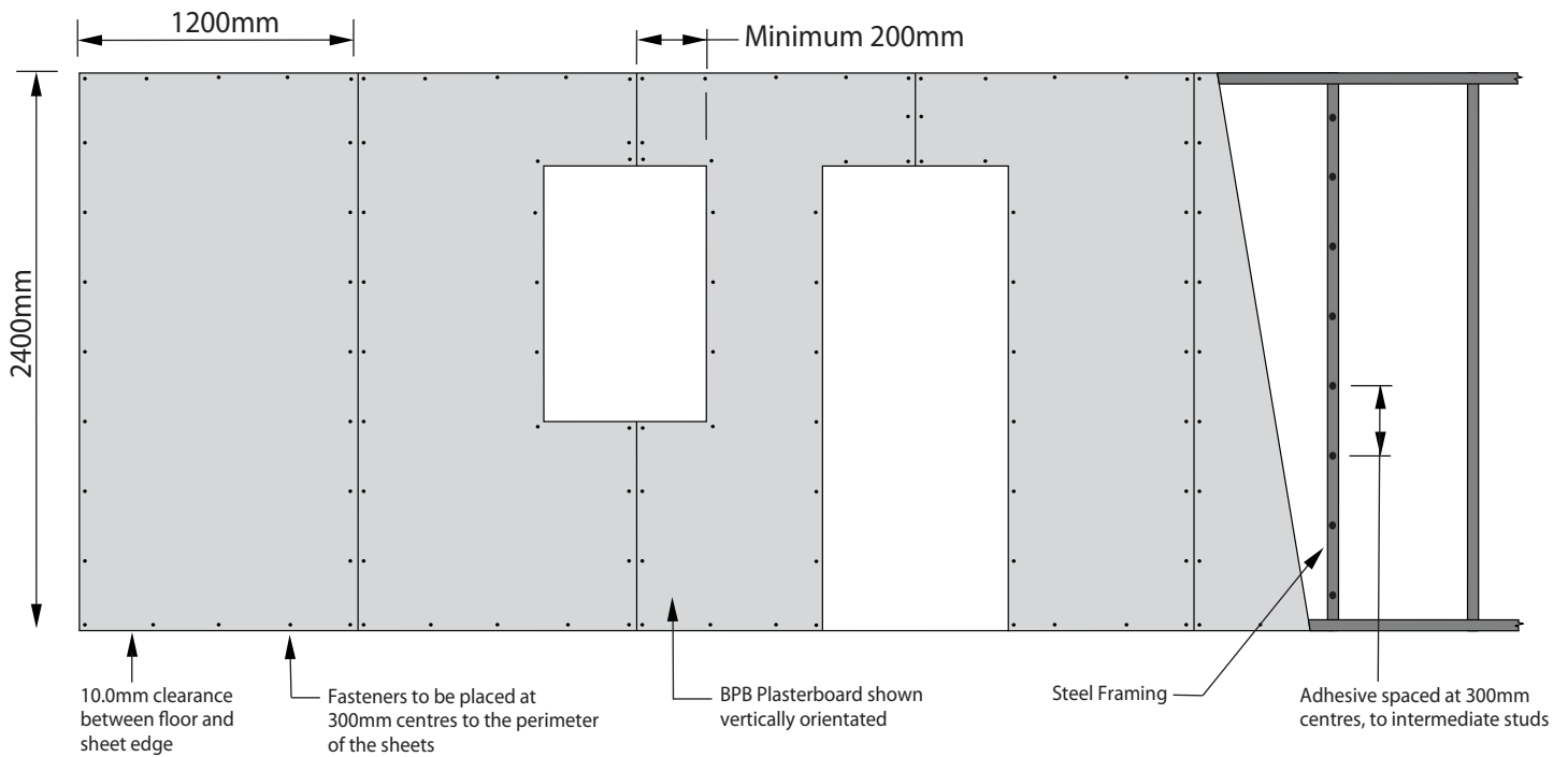
Typical construction wall layout - Sheets installed vertically
