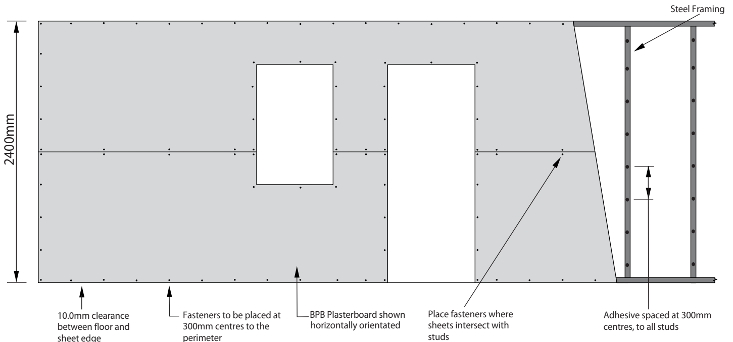
Typical construction wall layout - Sheets installed horizontally
